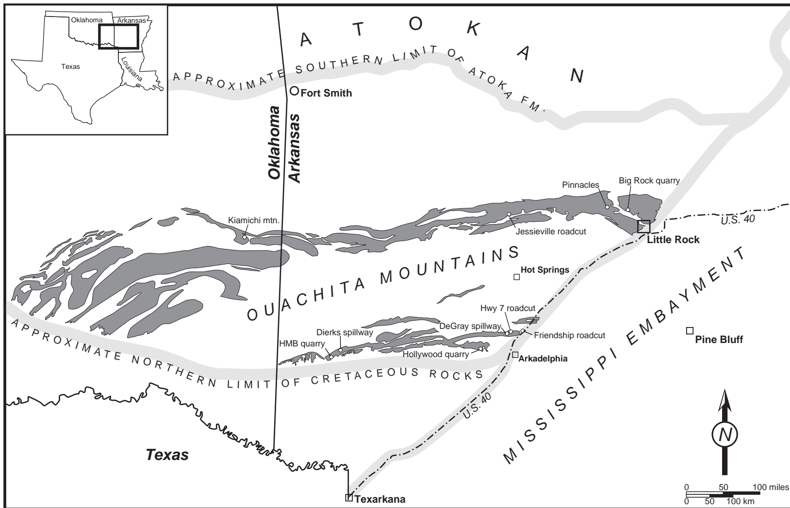
Figure 1. Jackfork Group outcrop map showing field localities. Dark shaded pattern is outcrop distribution
