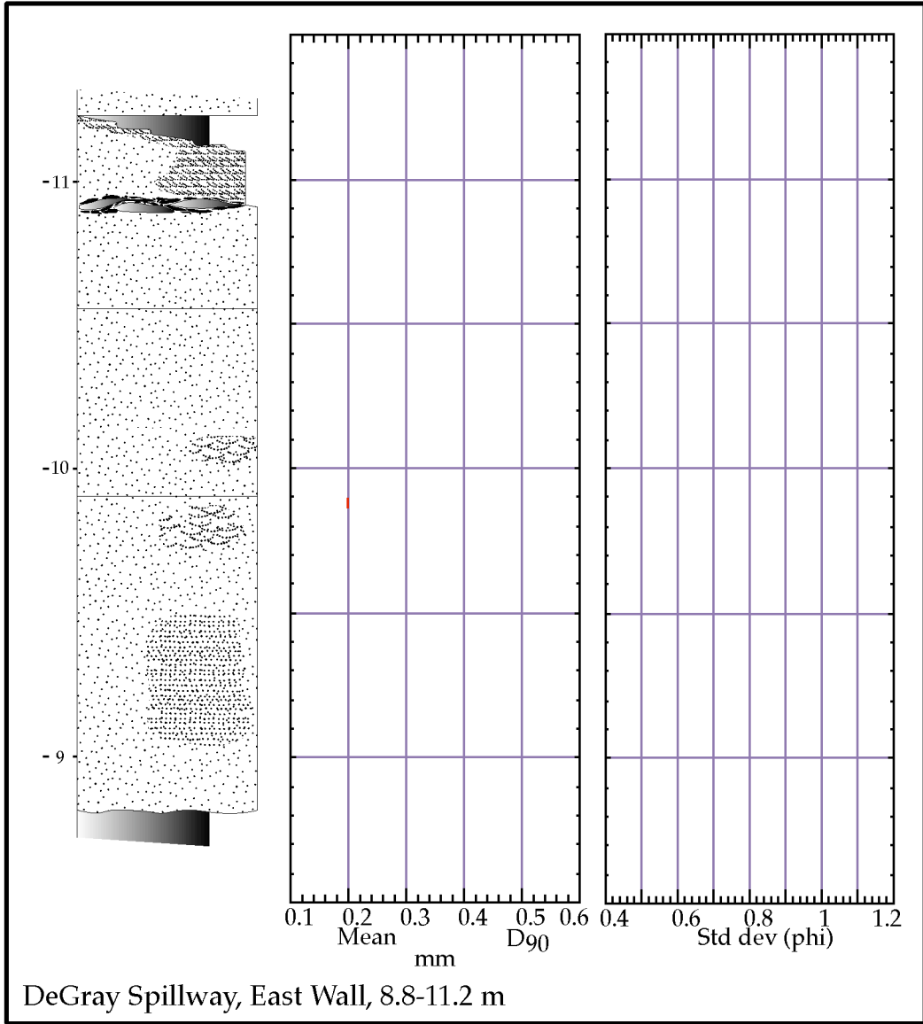
Figure 1. Lower DeGray spillway, 8.8 - 11.2 m
