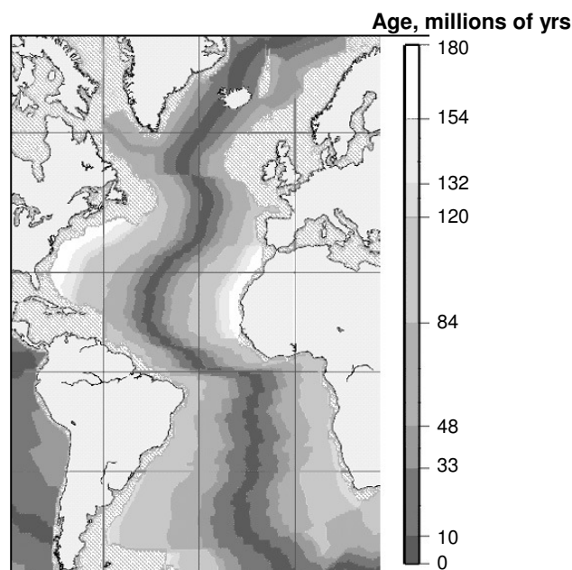
Map of the ages of the seafloor in the Atlantic Ocean
