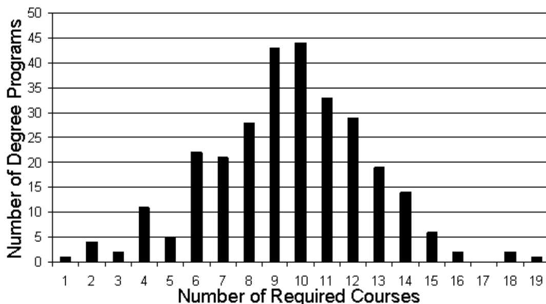
Figure 1. Distribution of the number of courses in the geology core as required by the 278 geology departments surveyed in the United States.
