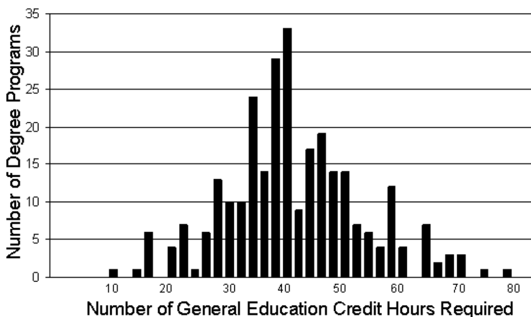
Figure 3. Distribution of the number of general education credit hours required by 283 geology departments surveyed in the United States (binning interval 2 credit hours).
