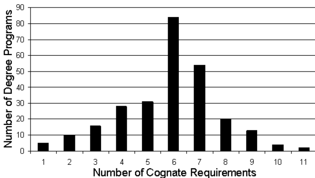
Figure 2. Distribution of the number of cognate science courses required by 267 geology departments surveyed in the United States.
