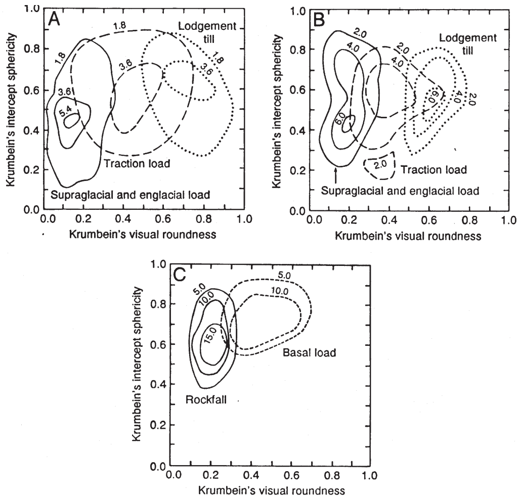
Modified from Gale and Hoare (1991). Boulton's (1978) modern glacial environments. A. Breidamerkurjokull, Iceland B. Sore Buchananisen, Spitzbergen and C. Dowdeswell et al., (1985) Grinnell Ice Cap, Baffin Island, Canada
