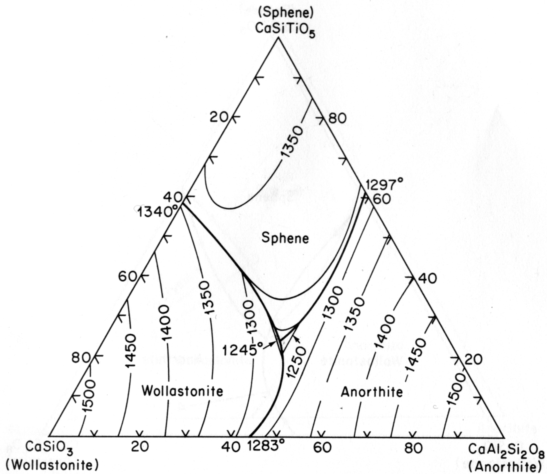
Figure 2. The ternary system wollastonite-anorthite-sphene with isothermal-contoured liquidus surface (after Nishioka, 1935).
