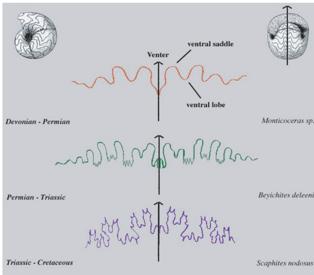
how paleontologists construct suture maps
