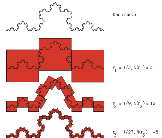
Measuring the Fractal Dimension of a Koch Curve
