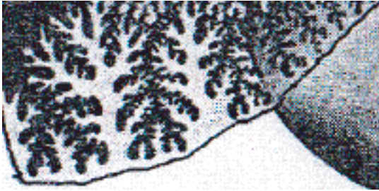
drawing of an ammonite suture
