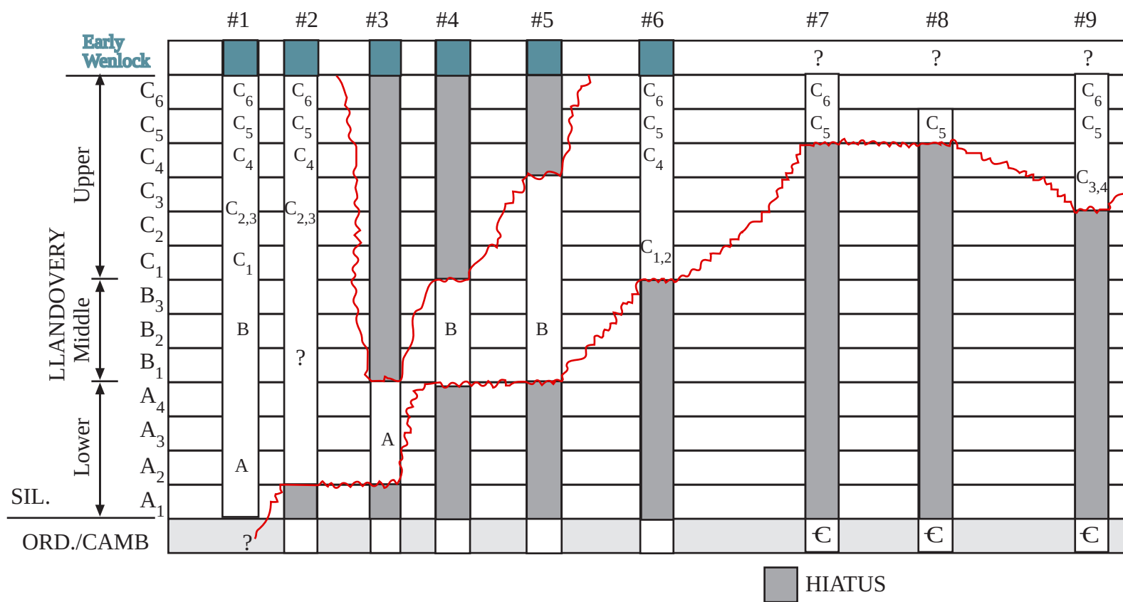
Time-stratigraphic Solution. (adapted from Ziegler et al., 1968 and from Miall, 1984)
